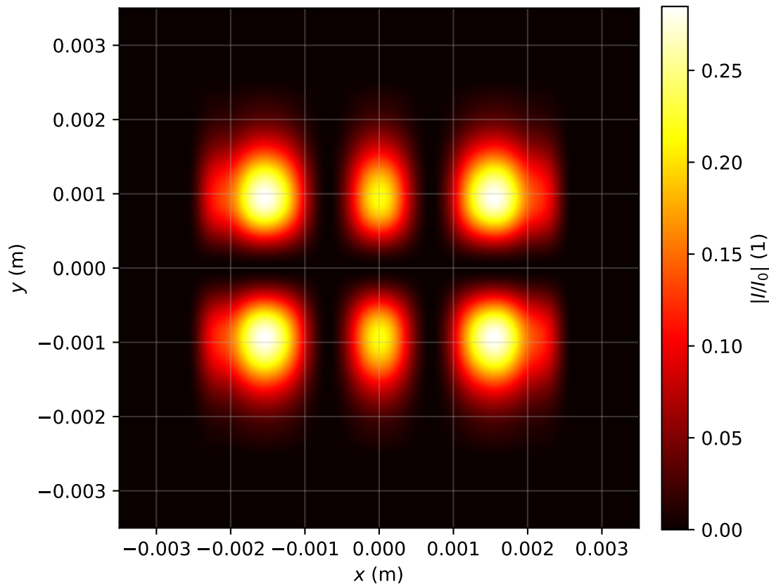
Intensity profile I(x, y, z = 3.344)/I_0 , P_{in}=0.5P_{cr} , artificial time
